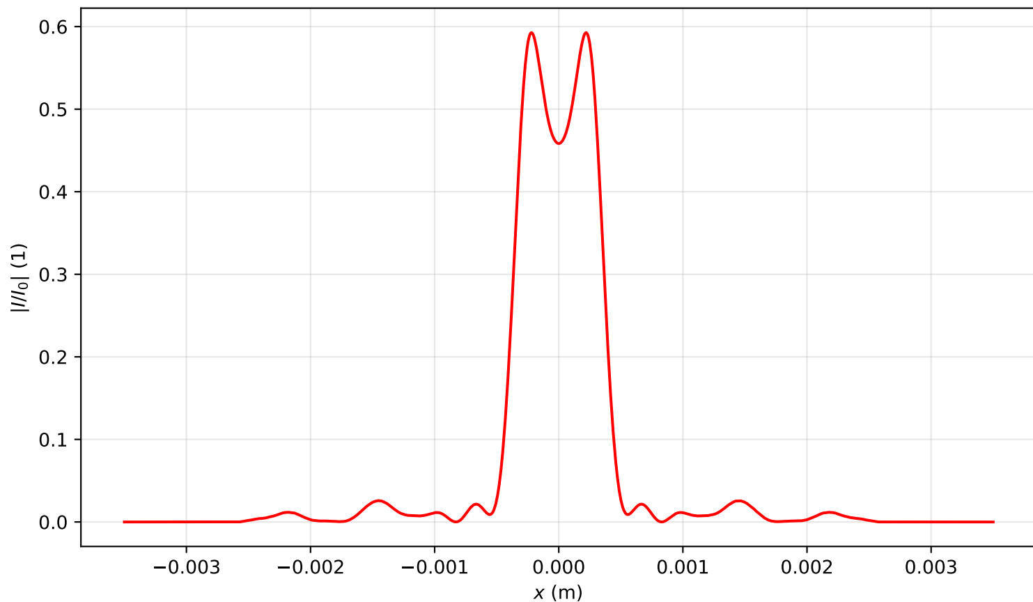
Intensity profile I(x, y = 0, z = 0.637)/I_0 , P_{in}=4.0P_{cr} , artificial time
